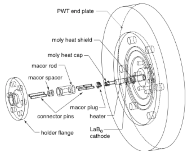
Figure 1: Schematic of thermionic cathode assembly.
