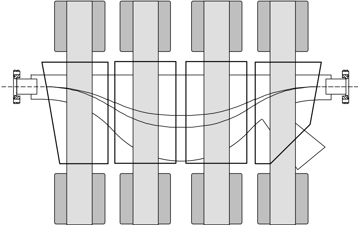
FIGURE 1. UCLA chicane system (5), showing path of two different energy electrons through magnetic compression system.
